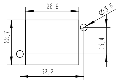
面板开孔图 Panel cul out
